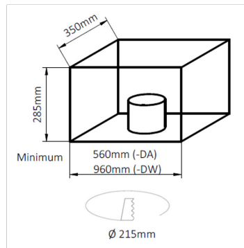
RDL AL G2 RGBW Minimum Ceiling Void and Ceiling Cut-out
