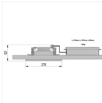
RDL AL G2 RGBW Drawing
